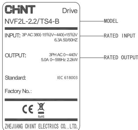
Figure 2.1.1 Nameplate Description
