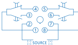
Figure 5 wiring diagram of JSS48A-2Z/JSS48A-G/JSS48A-P
