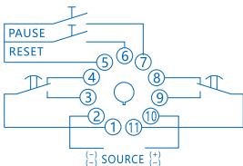
Figure 6 wiring diagram of JSS48A-11
